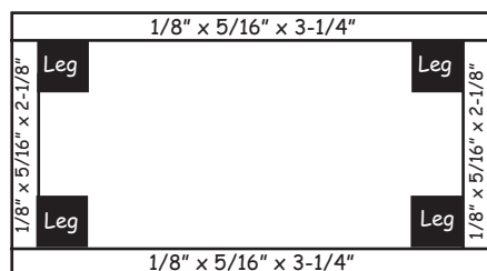
Top supports and legs for workbench (shown on underside of table).
